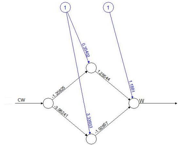
Figure 3. Model I ANNs Graph
