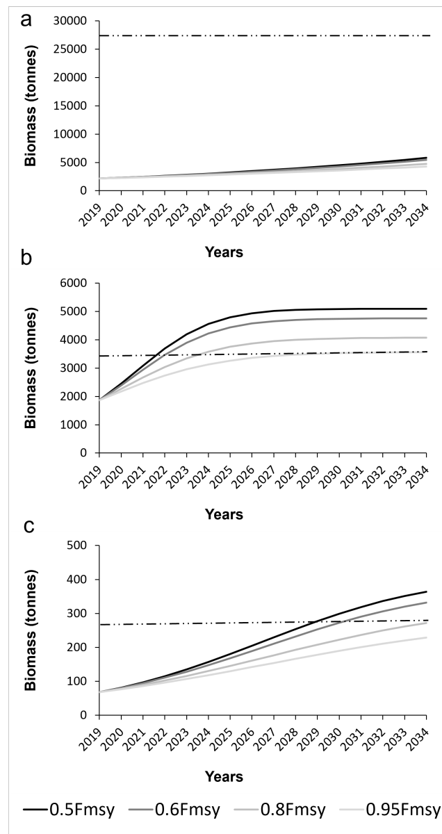
Figure 2. Future projection of biomass changes in depleted hake stock in (a) Marmara Sea, (b) Aegean Sea, and (c) Mediterranean Sea under four different fishing mortality scenarios as 0.5 F MSY , 0.6 F MSY , 0.8 F MSY and 0.95 F MSY values.
